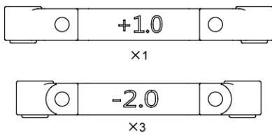
Suspension mount set (+1.0 / -2.0) 下擺臂座組 (+1.0 / -2.0) 230069
